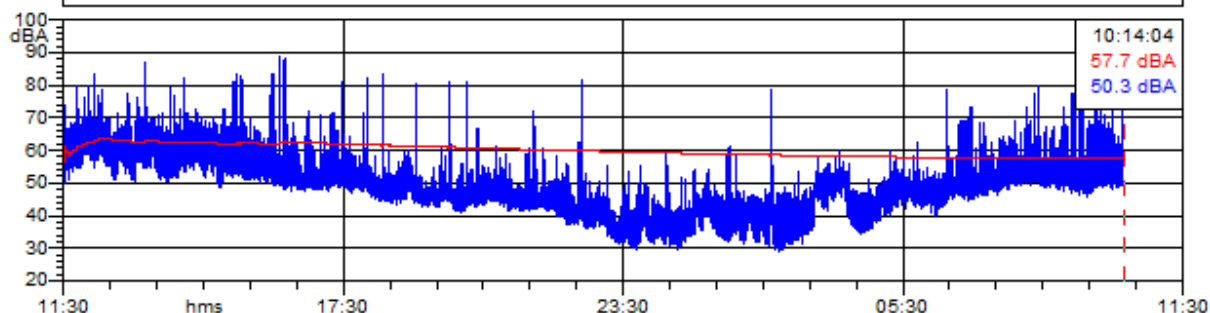
RLD6_24h - 1/3 Leq Spectrum + SLM - A
