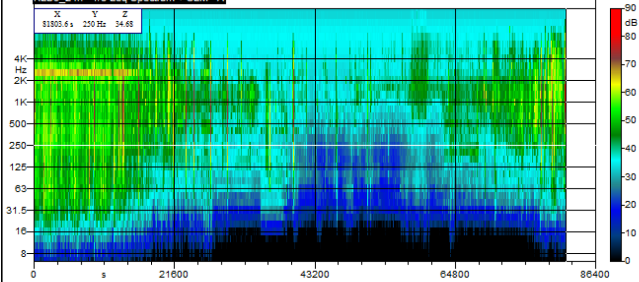
RLD6_24h - 1/3 Leq Spectrum + SLM - A
