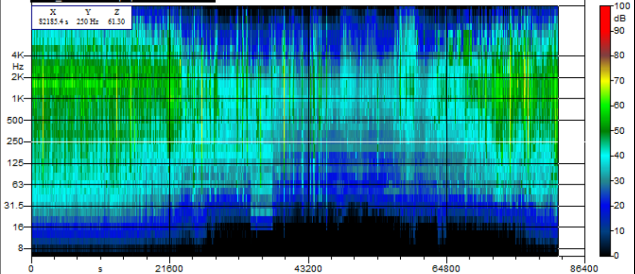
RLD4_24h - 1/3 Leq Spectrum + SLM - A
