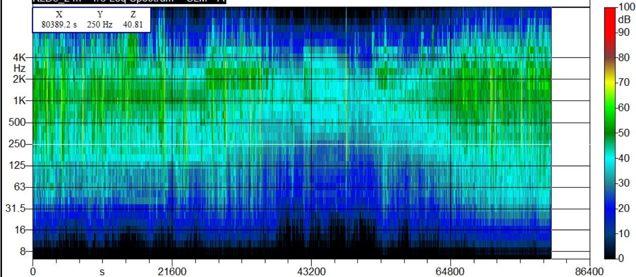
RLD5_24h - 1/3 Leq Spectrum + SLM - A
