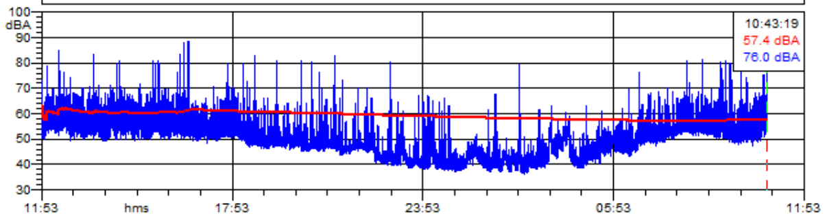
RLD4_24h - 1/3 Leq Spectrum + SLM - A
