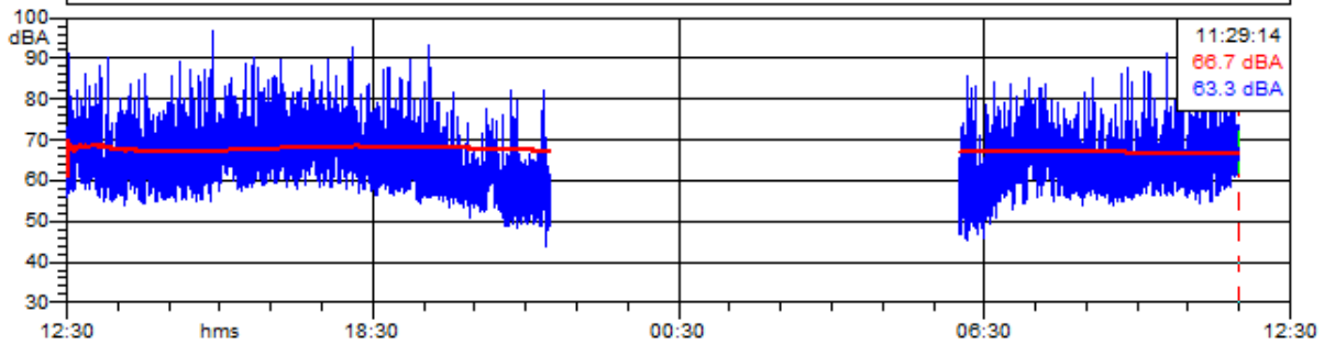
RLD3_diurno - 1/3 Leq Spectrum + SLM - A
